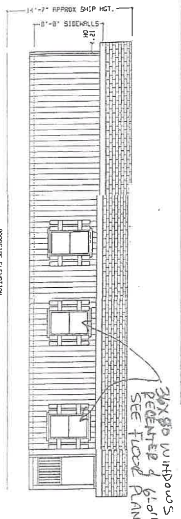
00095 SIDE ELEVATION
